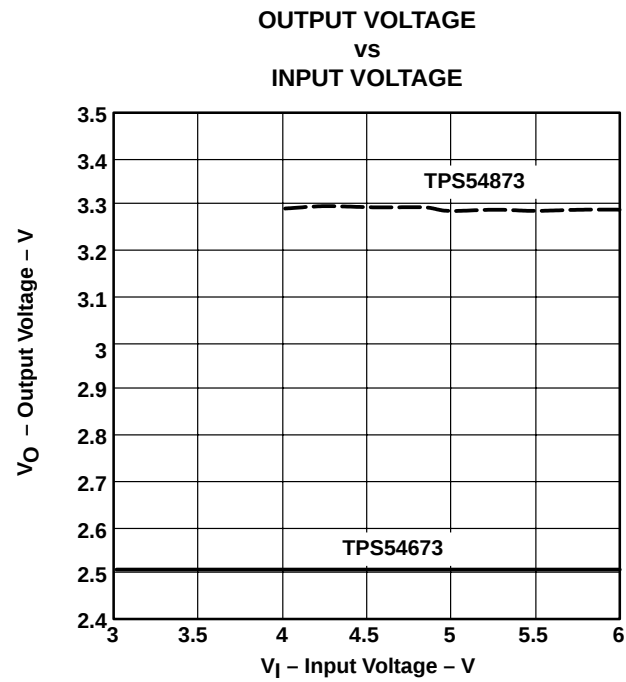
Figure 2–6. Line Regulation
