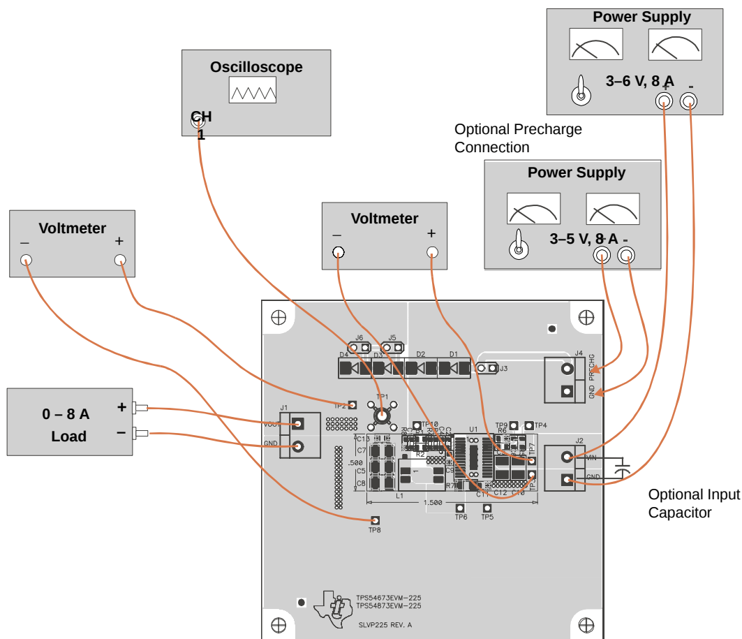
Figure 2–1. Connection Diagram
