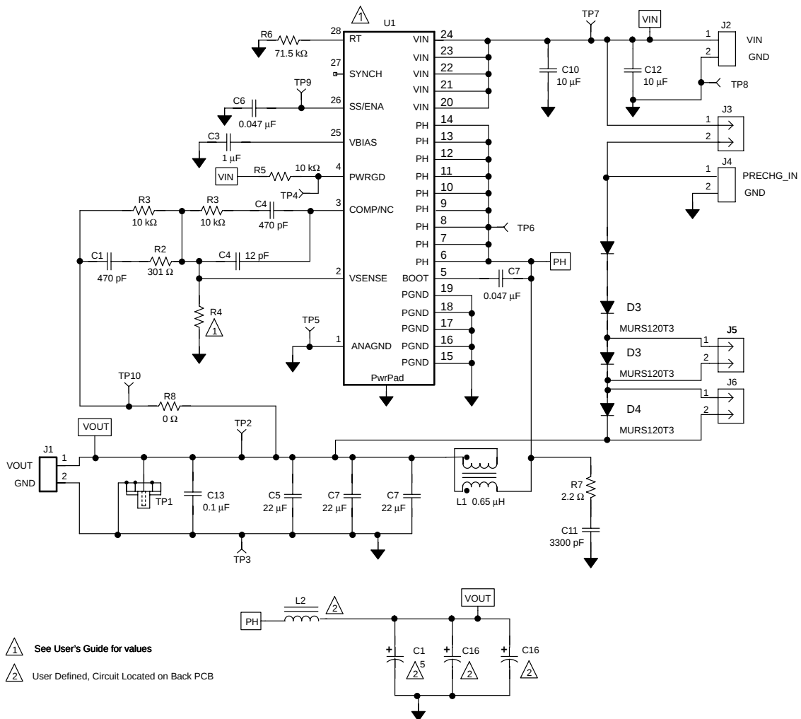
Figure 4–1. TPS54x73EVM-225 Schematic
